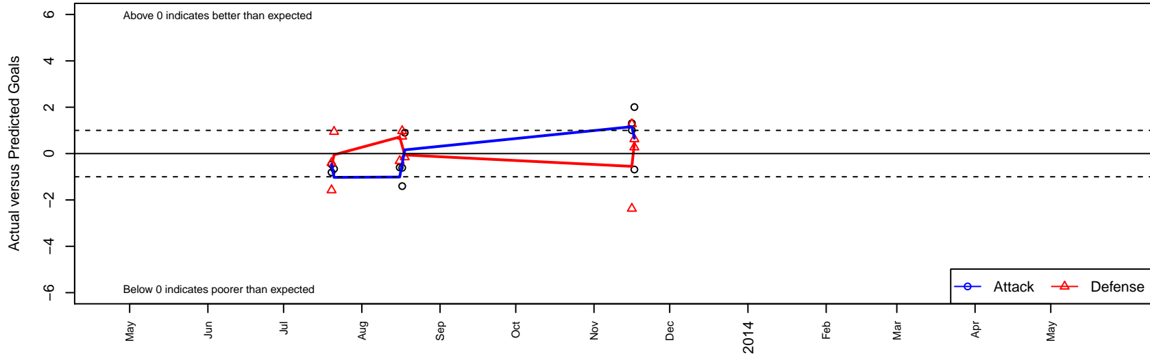
THSSP Earthquakes G00 Dots are actual minus expected GF (blue circles) and GA (red triangles). Blue line is smoothed change in attack strength. Red is smoothed change in defense strength.
